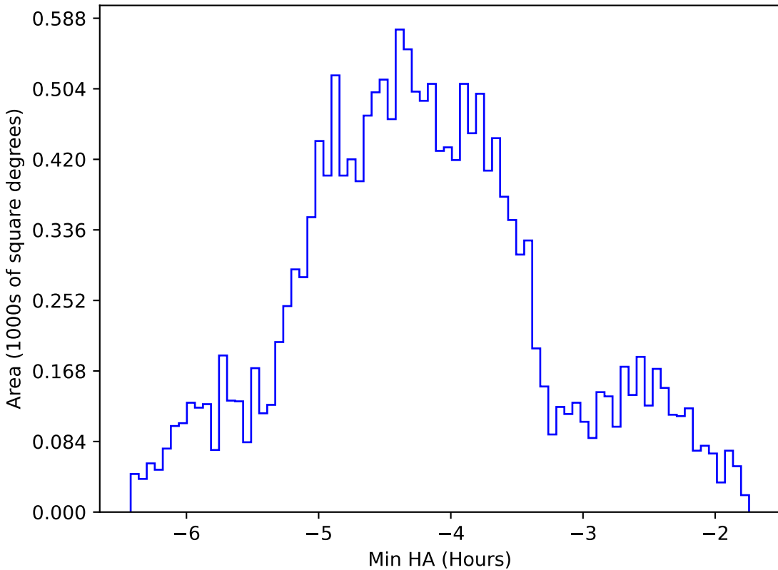
ddf_acor_sf15_lsf40_lsr50_v3.4_10yrs WFD g band: Min HA
