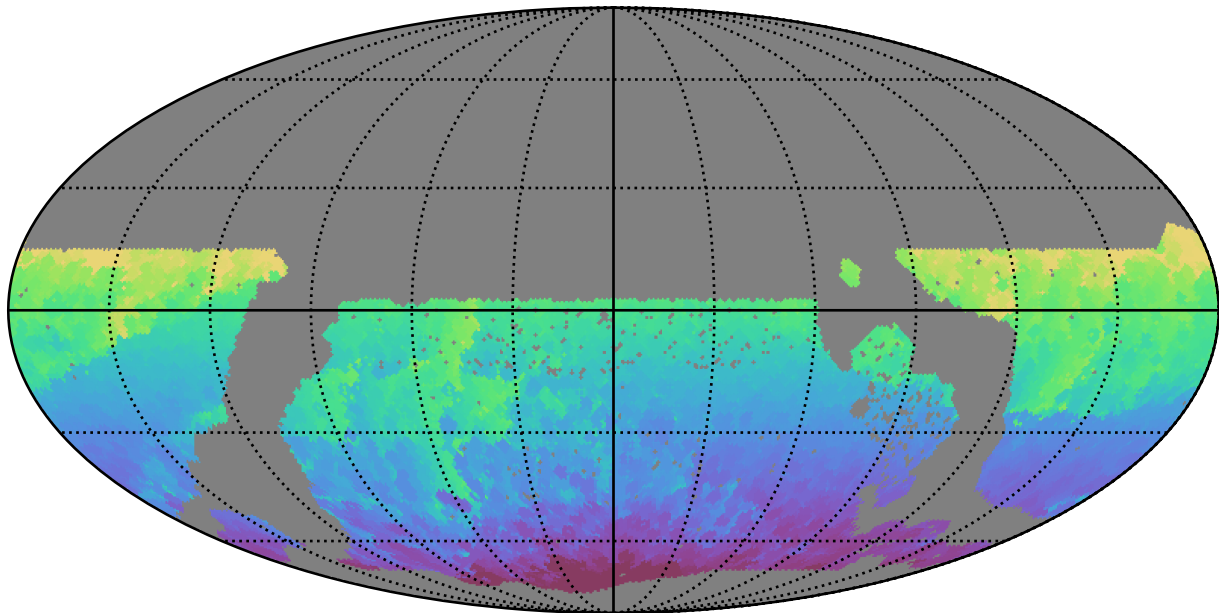
ddf_acor_sf15_lsf40_lsr50_v3.4_10yrs WFD all bands: Min HA
