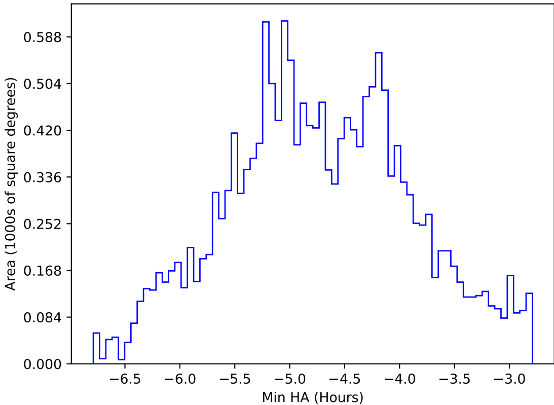
ddf_acor_sf15_ls40_lsr50_v3.4_10yrs WFD all bands: Min HA
