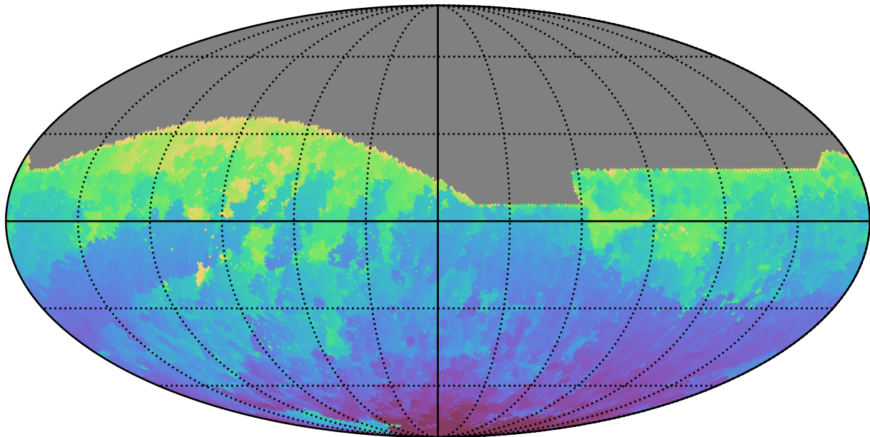
ddf_acor_sf15_lsf40_lsr50_v3.4_10yrs All sky z band: Min HA
