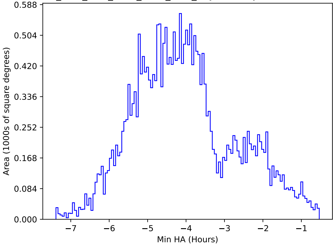
ddf_acor_sf15_lsf40_lsr50_v3.4_10yrs All sky z band: Min HA
