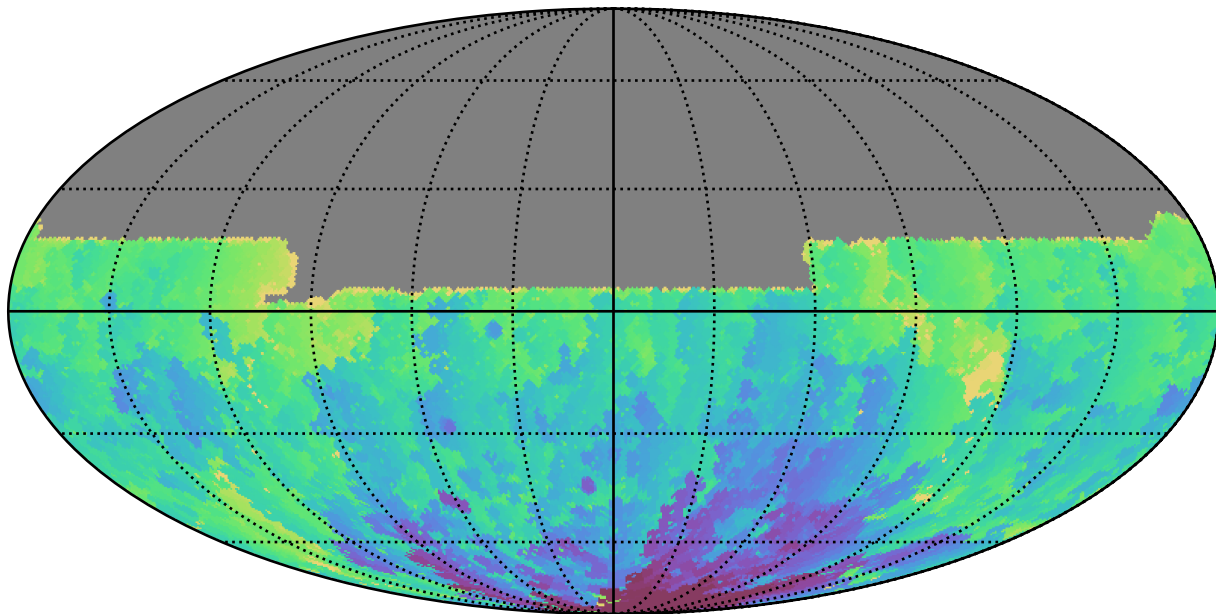
ddf_acor_sf15_lsf40_lsr50_v3.4_10yrs All sky u band: Min HA
