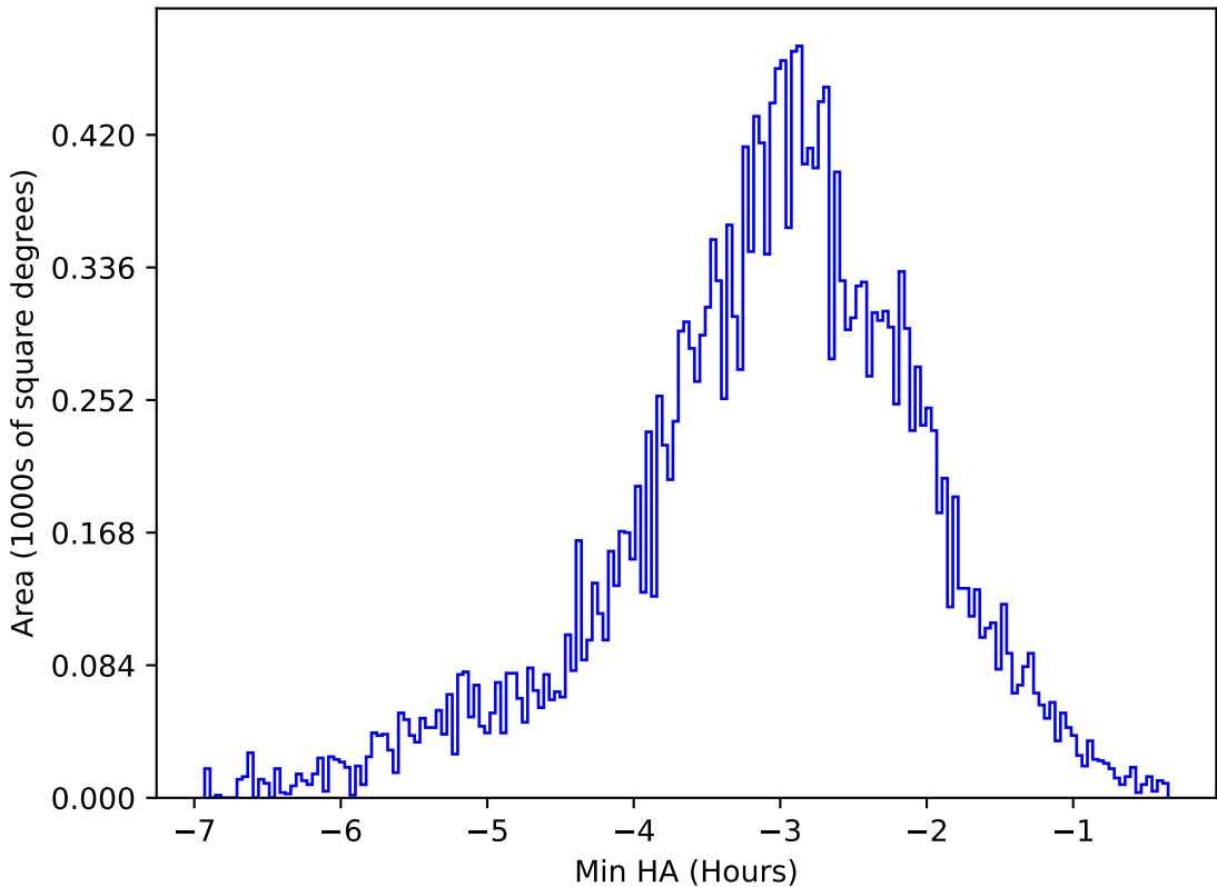
ddf_acor_sf15_lsf40_lsr50_v3.4_10yrs All sky u band: Min HA
