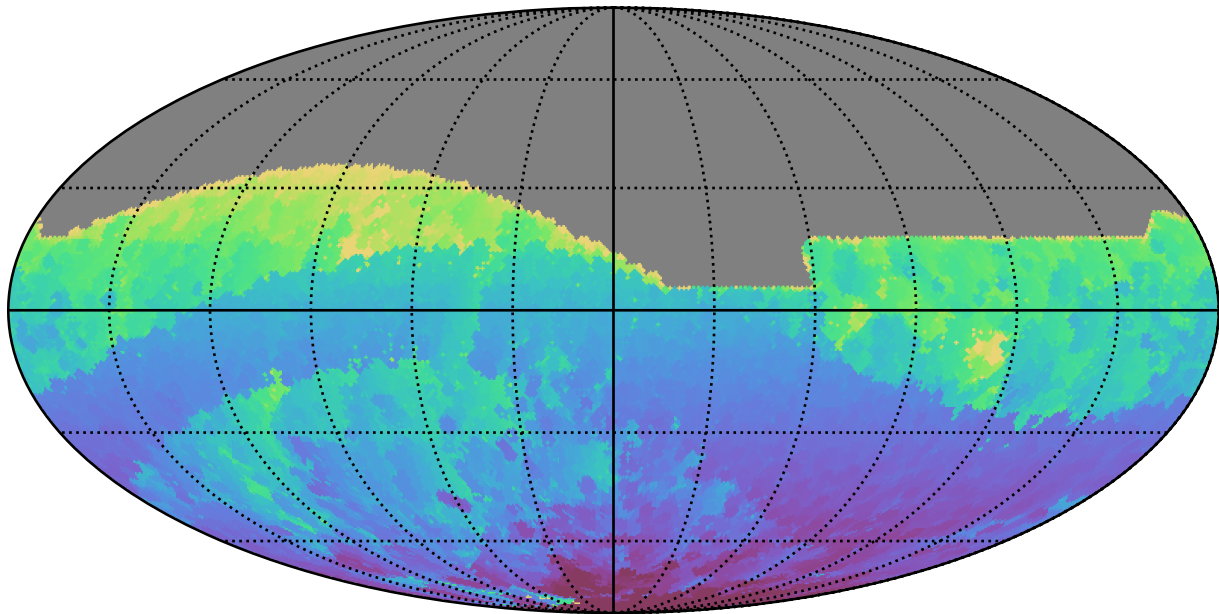
ddf_acor_sf15_lsf40_lsr50_v3.4_10yrs All sky r band: Min HA
