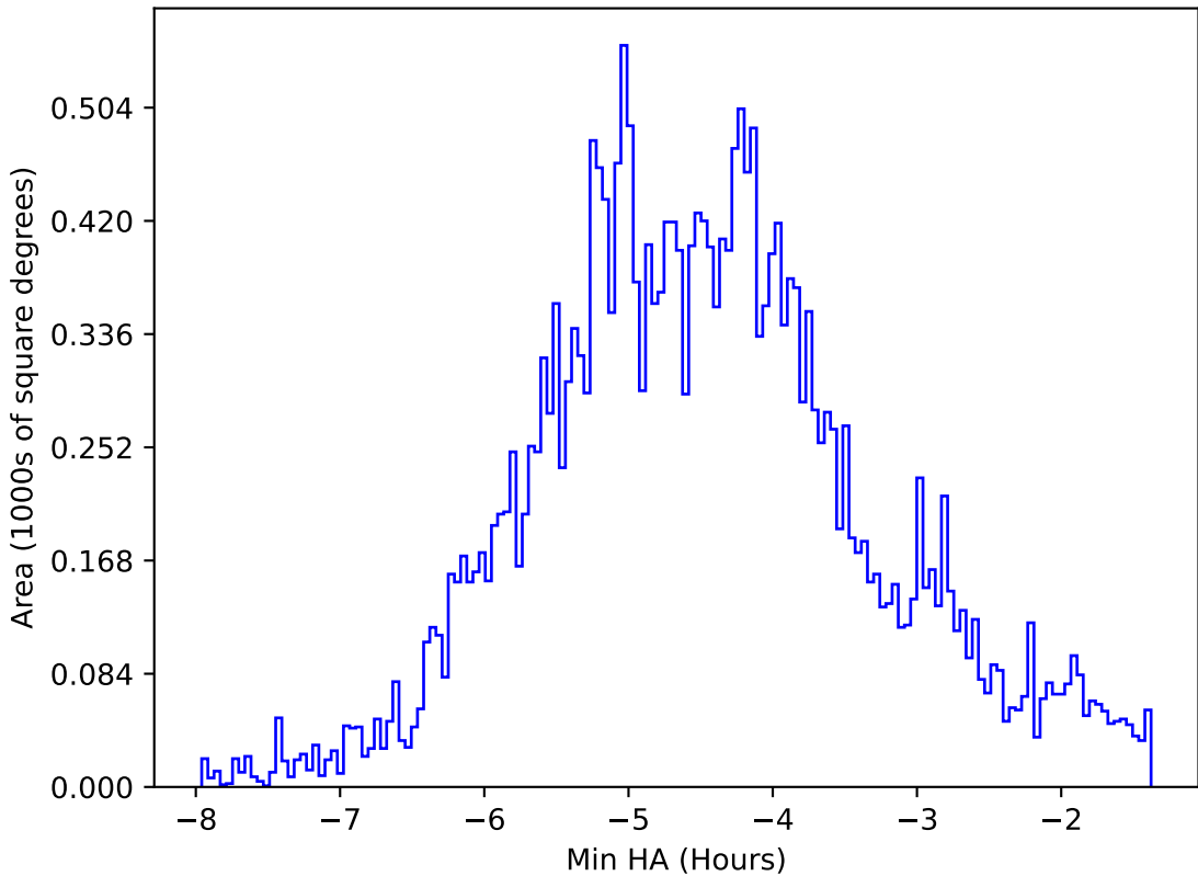
ddf_acor_sf15_lsf40_lsr50_v3.4_10yrs All sky all bands: Min HA
