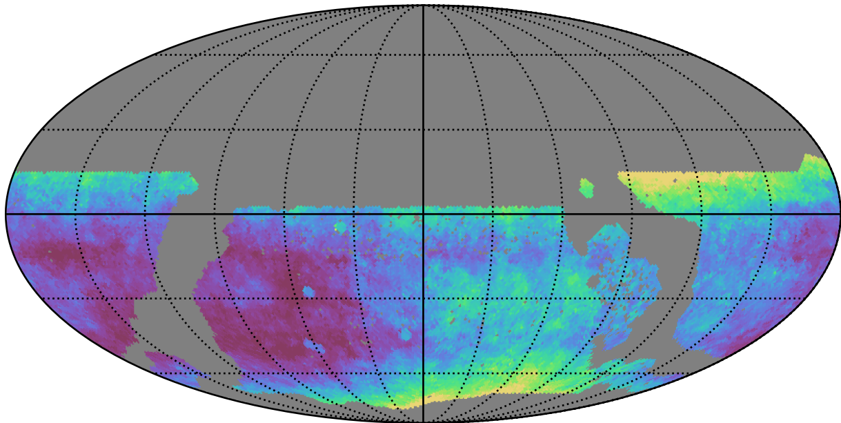
ddf_acor_sf15_lsf40_lsr50_v3.4_10yrs WFD i band: Median seeingEff
