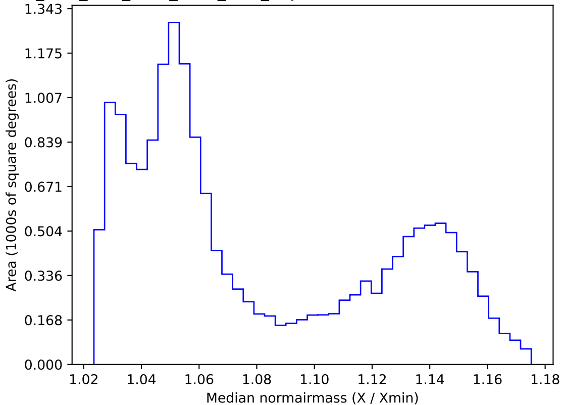
ddf_acor_sf15_lsf40_lsr50_v3.4_10yrs WFD all bands: Median normairmass
