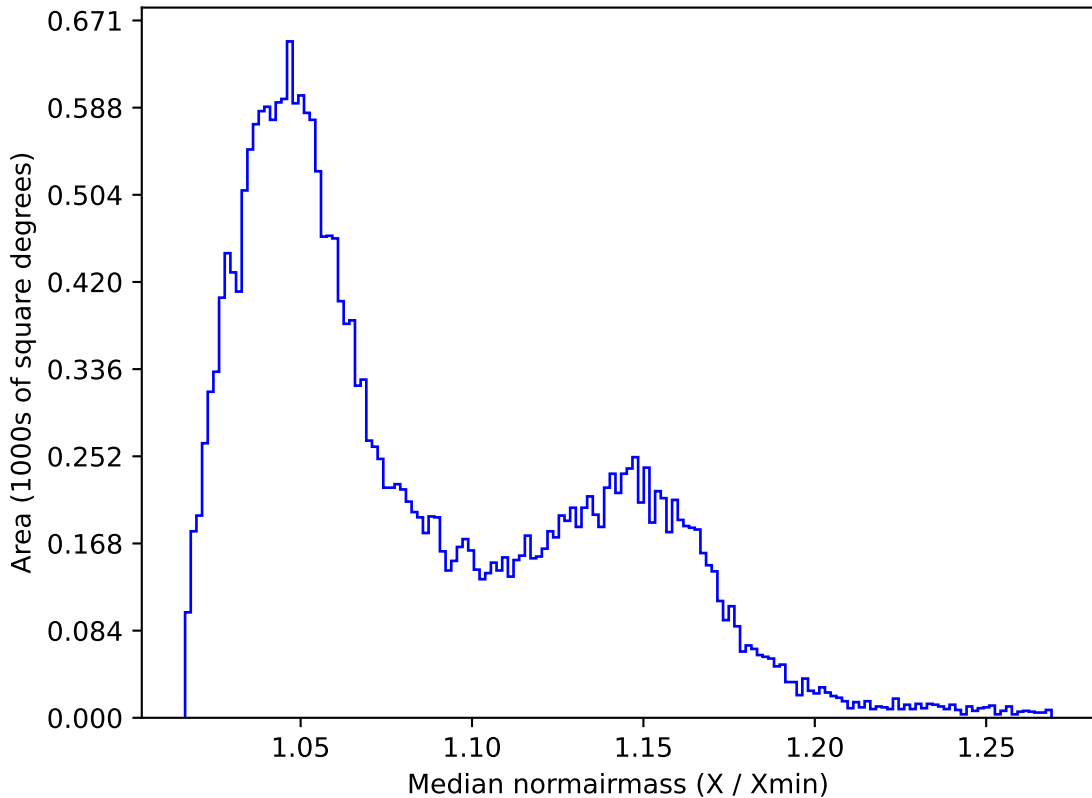
ddf_acor_sf15_lsf40_lsr50_v3.4_10yrs All sky z band: Median normairmass
