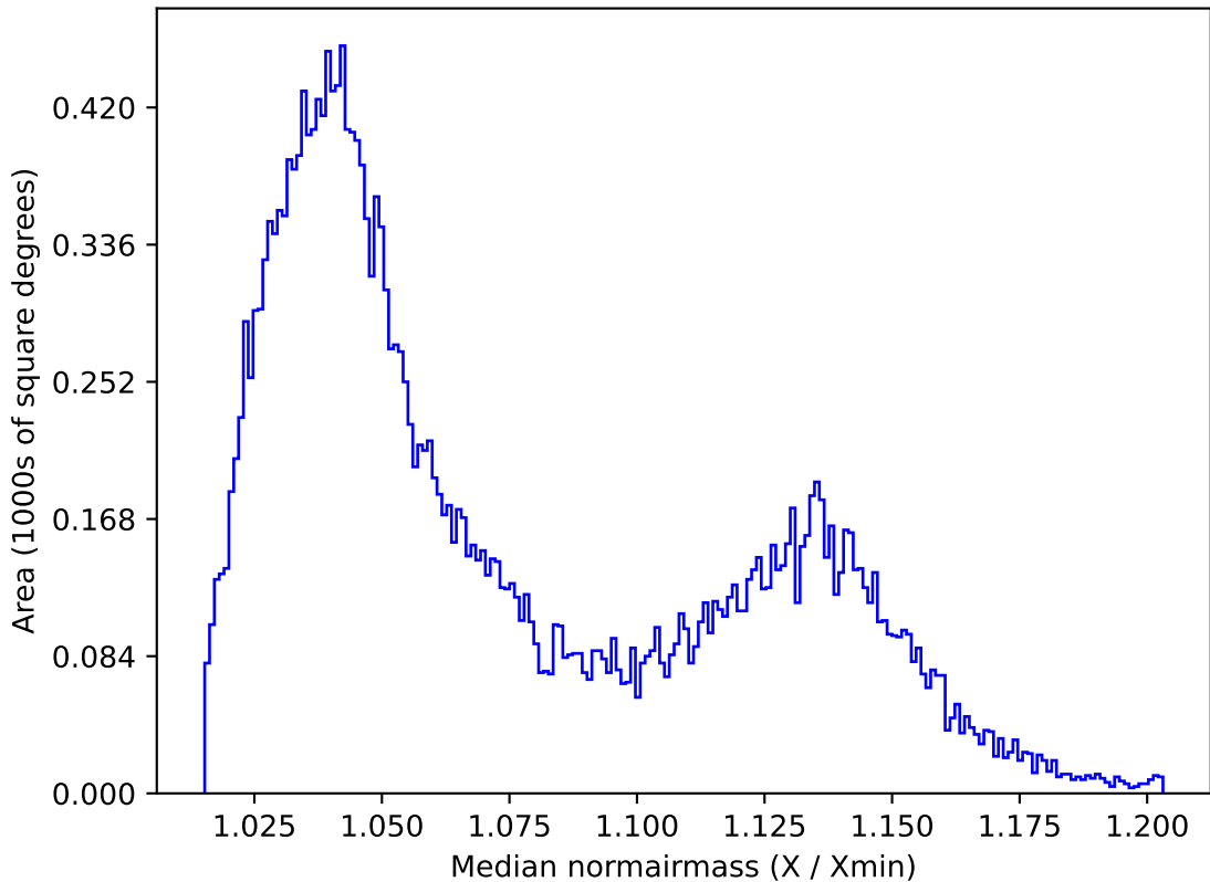
ddf_acor_sf15_lsf40_lsr50_v3.4_10yrs All sky i band: Median normairmass
