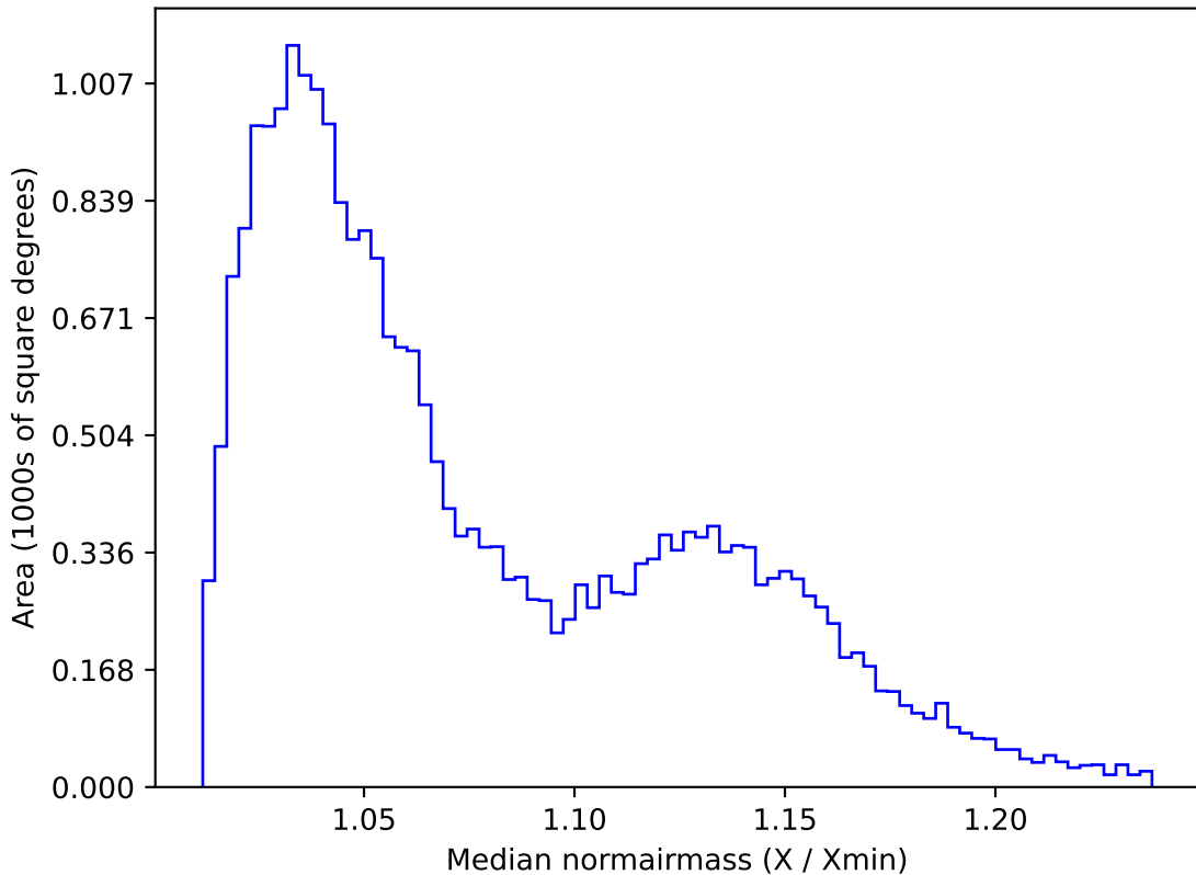
ddf_acor_sf15_lsf40_lsr50_v3.4_10yrs All sky g band: Median normairmass
