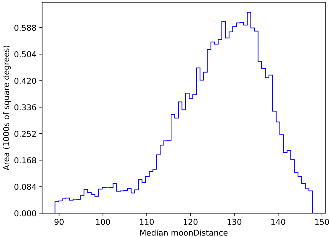
ddf_acor_sf15_ls40_lsr50_v3.4_10yrs WFD u band: Median moonDistance
