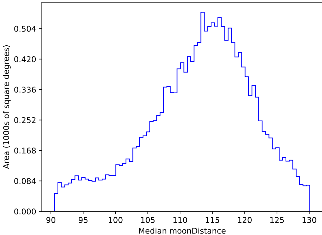
ddf_acor_sf15_lsf40_lsr50_v3.4_10yrs WFD r band: Median moonDistance
