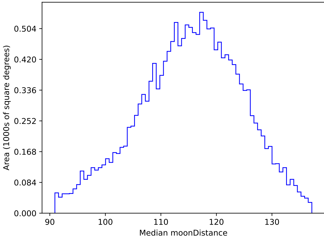
ddf_acor_sf15_ls40_lsr50_v3.4_10yrs WFD g band: Median moonDistance
