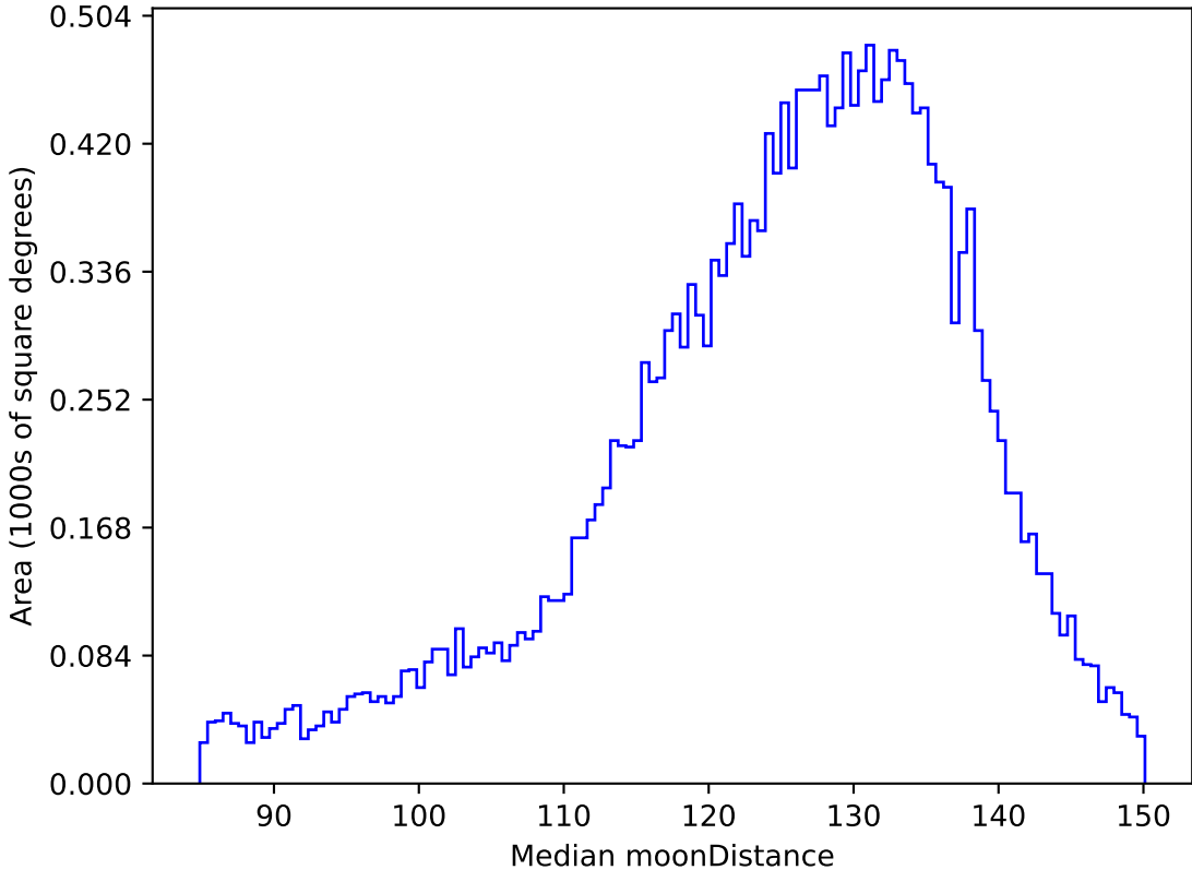
ddf_acor_sf15_lsf40_lsr50_v3.4_10yrs All sky u band: Median moonDistance
