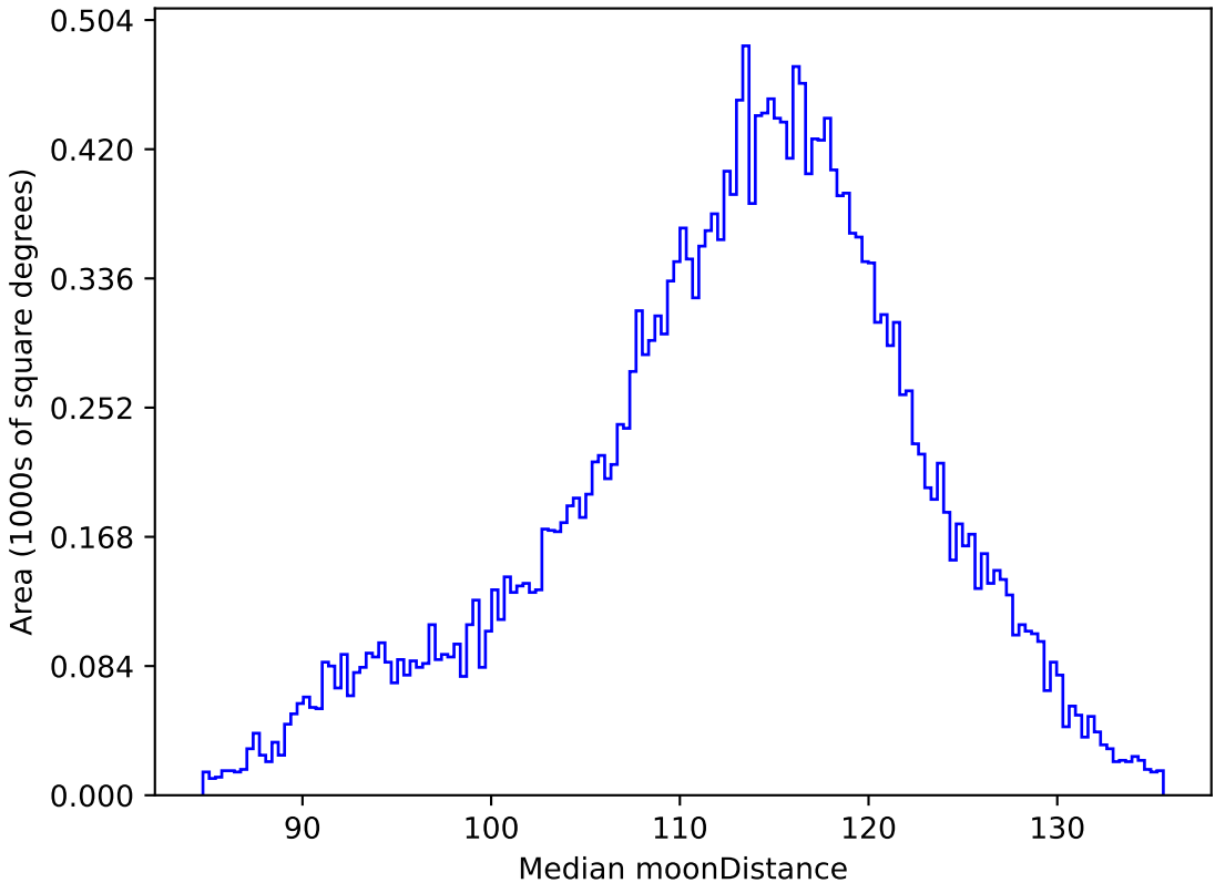
ddf_acor_sf15_lsf40_lsr50_v3.4_10yrs All sky r band: Median moonDistance
