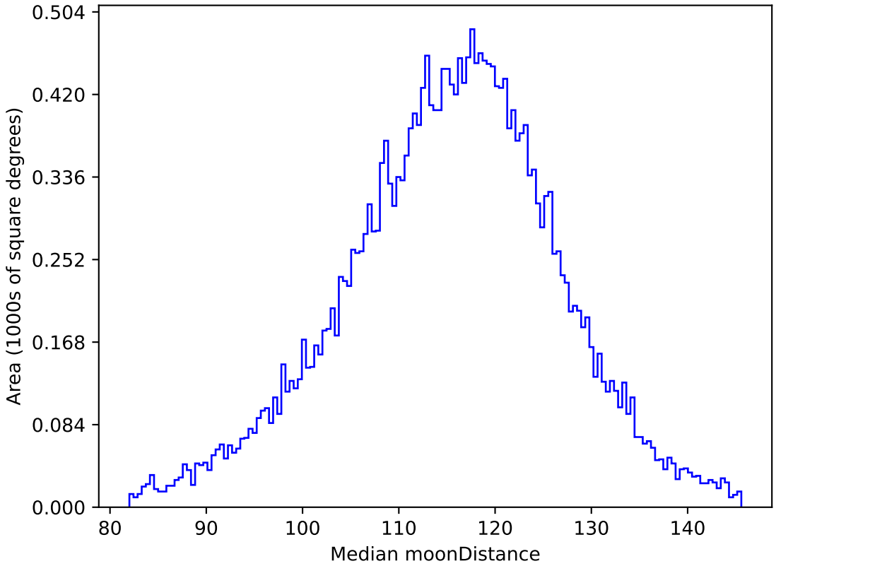
ddf_acor_sf15_lsf40_lsr50_v3.4_10yrs All sky g band: Median moonDistance
