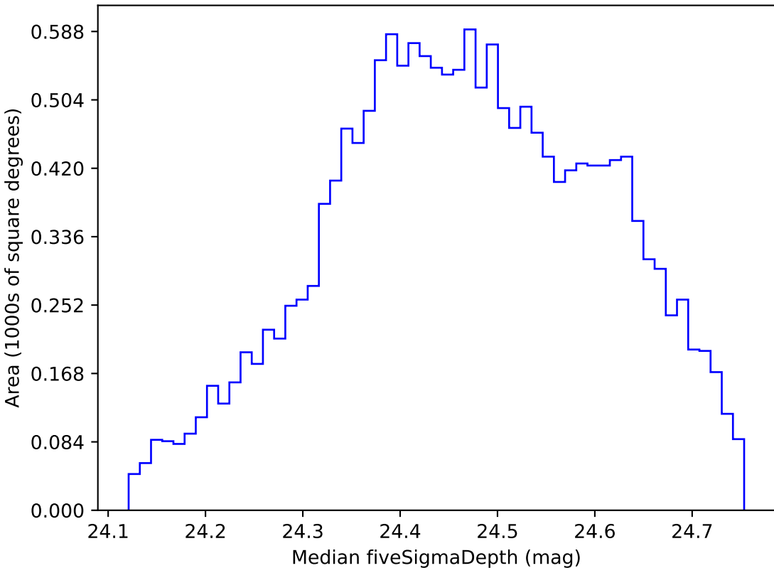
ddf_acor_sf15_lsf40_lsr50_v3.4_10yrs WFD g band: Median fiveSigmaDepth
