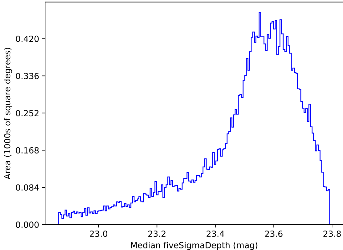
ddf_acor_sf15_lsf40_lsr50_v3.4_10yrs All sky i band: Median fiveSigmaDepth
