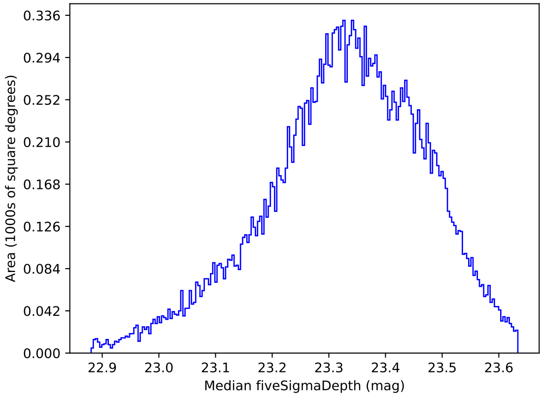
ddf_acor_sf15_lsf40_lsr50_v3.4_10yrs All sky all bands: Median fiveSigmaDepth
