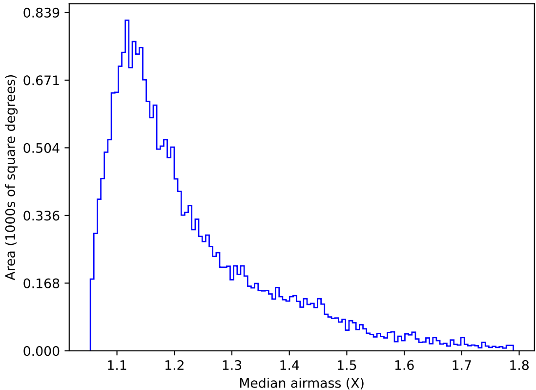
ddf_acor_sf15_lsf40_lsr50_v3.4_10yrs Yr 1 u band: Median airmass
