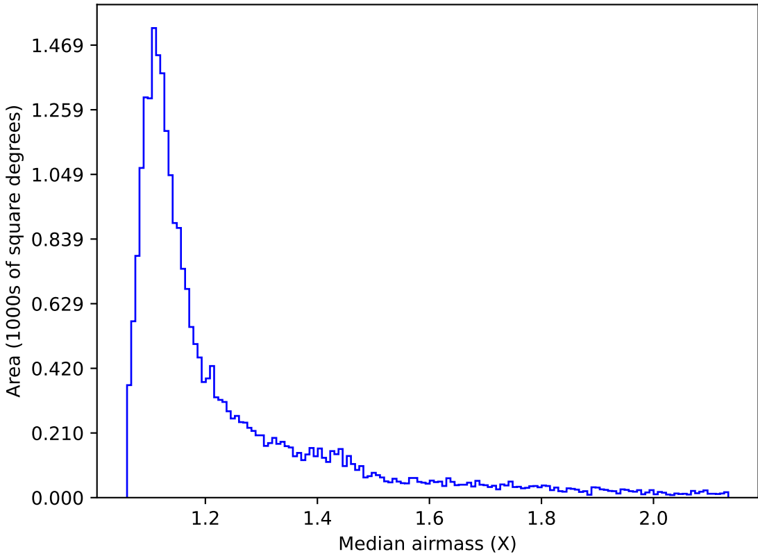
ddf_acor_sf15_lsf40_lsr50_v3.4_10yrs Yr 1 i band: Median airmass
