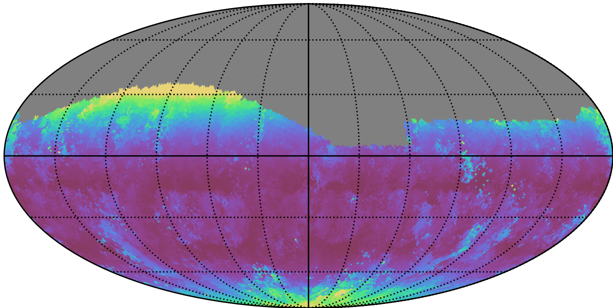
ddf_acor_sf15_lsf40_lsr50_v3.4_10yrs Yr 1 g band: Median airmass
