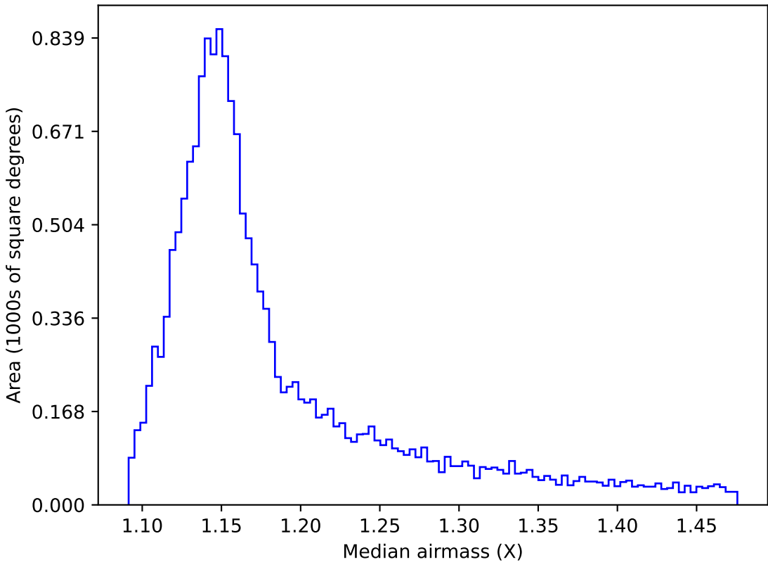
ddf_acor_sf15_lsf40_lsr50_v3.4_10yrs WFD y band: Median airmass
