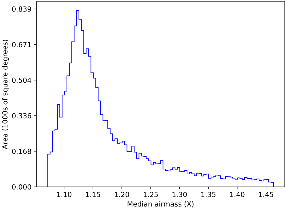
ddf_acor_sf15_lsf40_lsr50_v3.4_10yrs WFD u band: Median airmass
