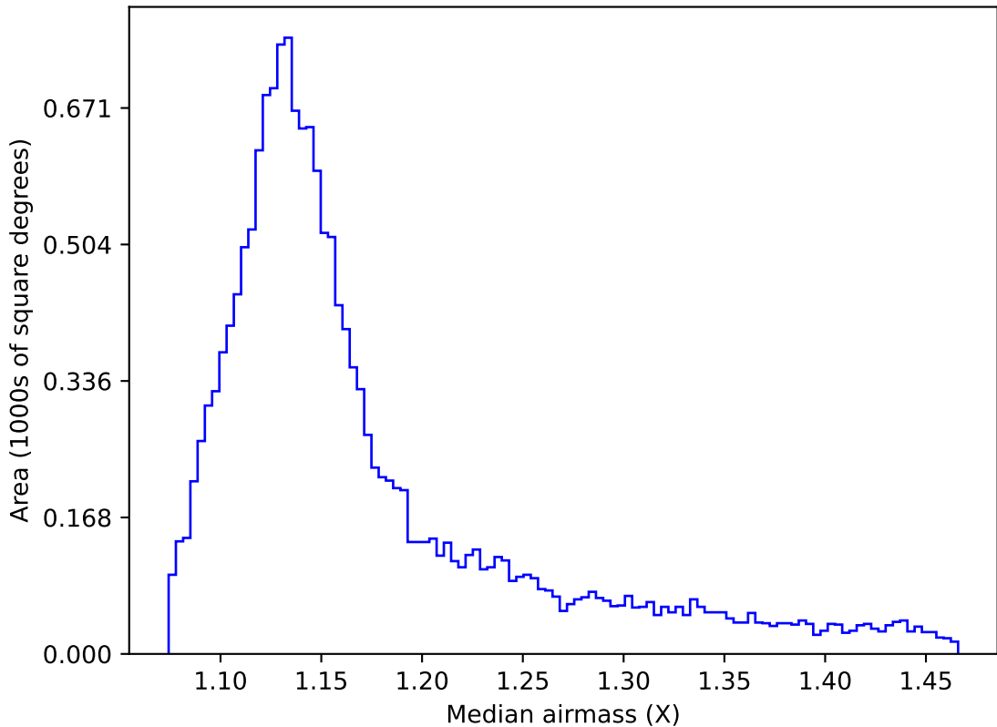
ddf_acor_sf15_lsf40_lsr50_v3.4_10yrs WFD r band: Median airmass
