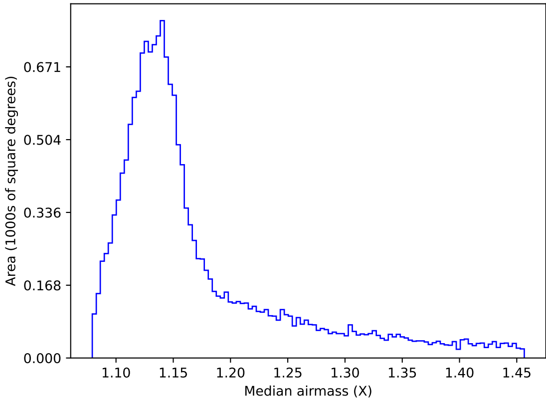
ddf_acor_sf15_lsf40_lsr50_v3.4_10yrs WFD i band: Median airmass
