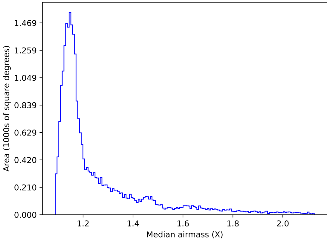
ddf_acor_sf15_lsf40_lsr50_v3.4_10yrs All sky z band: Median airmass
