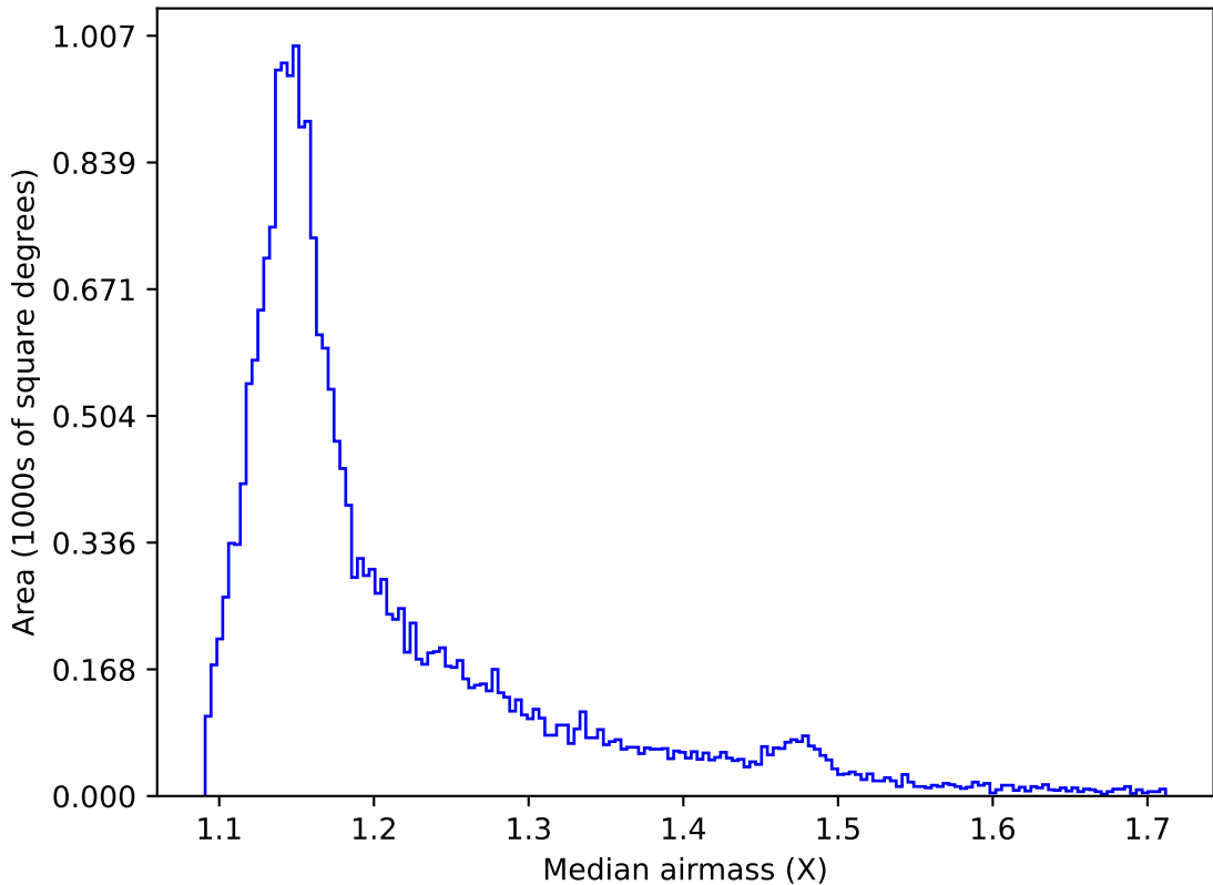
ddf_acor_sf15_lsf40_lsr50_v3.4_10yrs All sky y band: Median airmass
