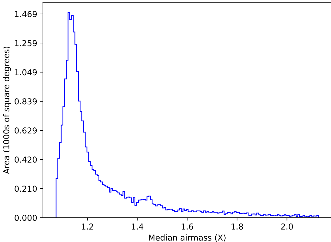
ddf_acor_sf15_lsf40_lsr50_v3.4_10yrs All sky g band: Median airmass
