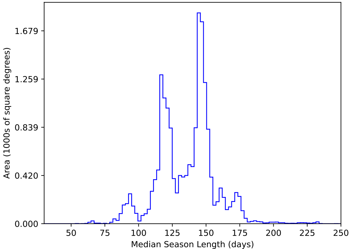
ddf_acor_sf15_lsf40_lsr50_v3.4_10yrs WFD y band: Median Season Length
