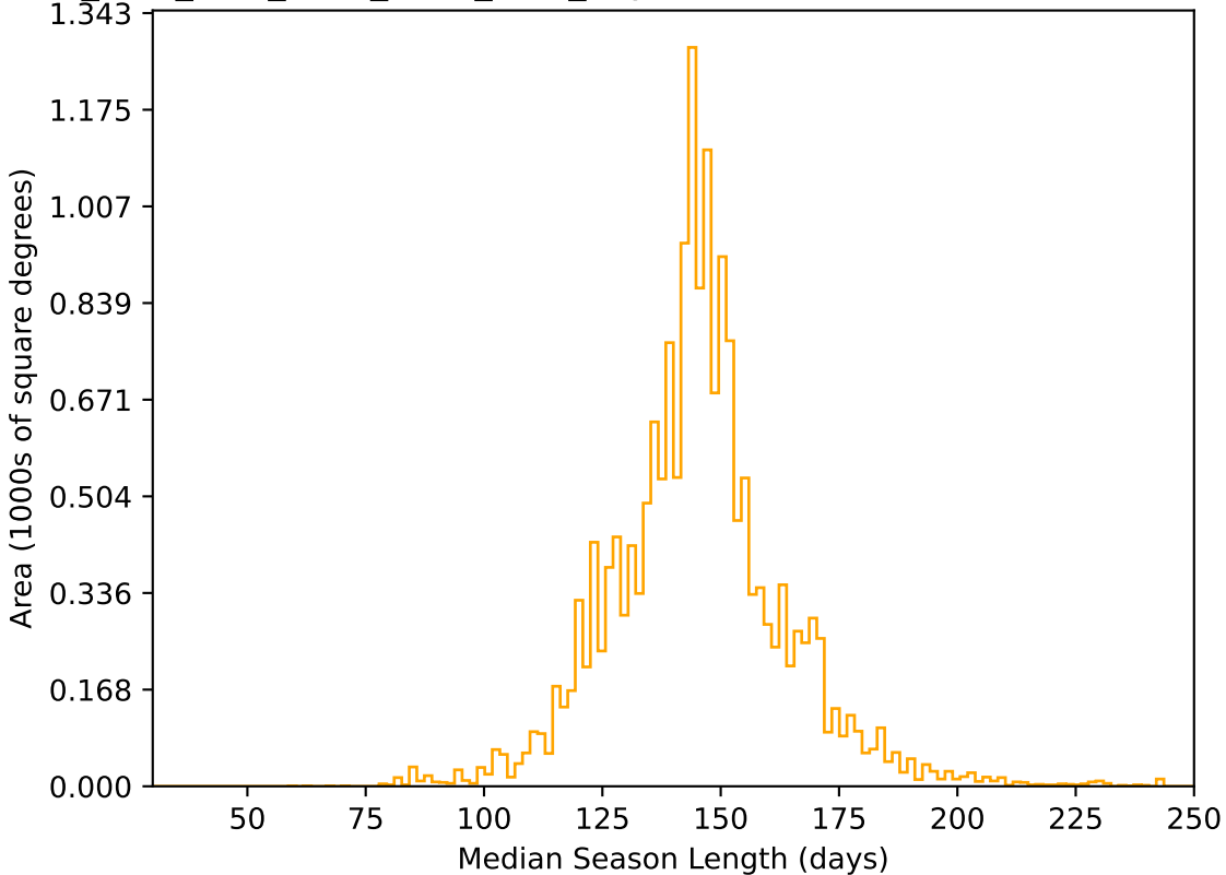
ddf_acor_sf15_lsf40_lsr50_v3.4_10yrs WFD r band: Median Season Length
