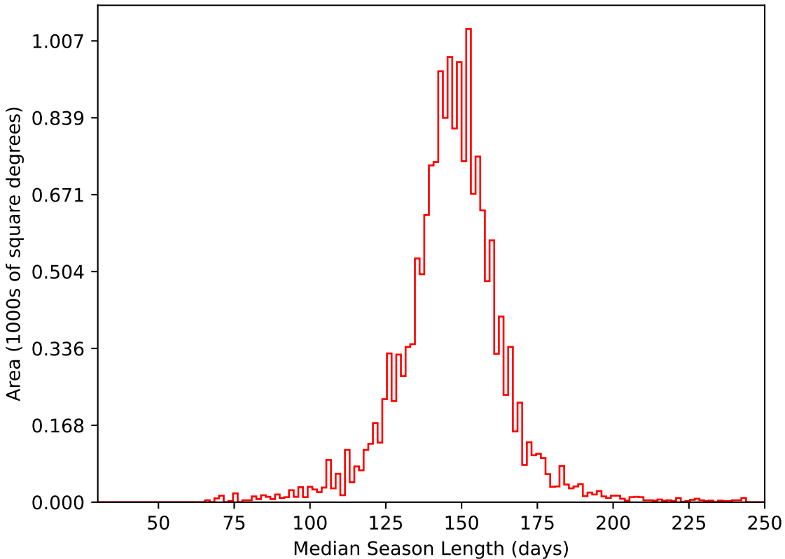
ddf_acor_sf15_lsf40_lsr50_v3.4_10yrs WFD i band: Median Season Length
