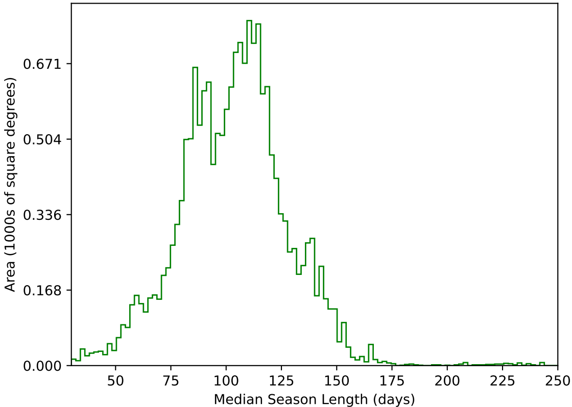
ddf_acor_sf15_lsf40_lsr50_v3.4_10yrs WFD g band: Median Season Length
