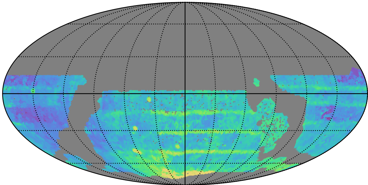
ddf_acor_sf15_lsf40_lsr50_v3.4_10yrs WFD all bands: Median Season Length
