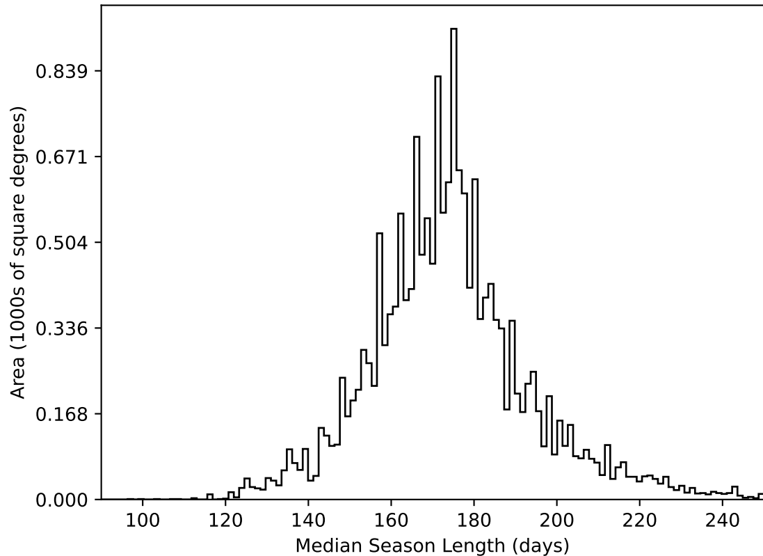
ddf_acor_sf15_lsf40_lsr50_v3.4_10yrs WFD all bands: Median Season Length
