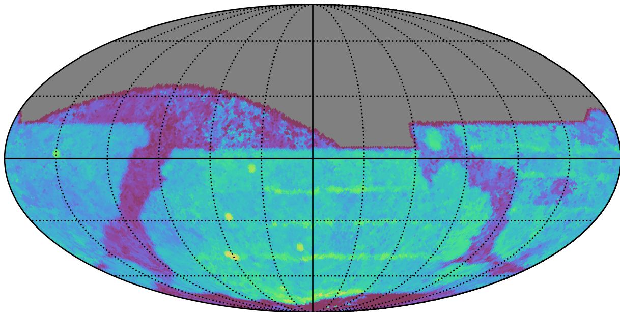
ddf_acor_sf15_lsf40_lsr50_v3.4_10yrs All sky z band: Median Season Length
