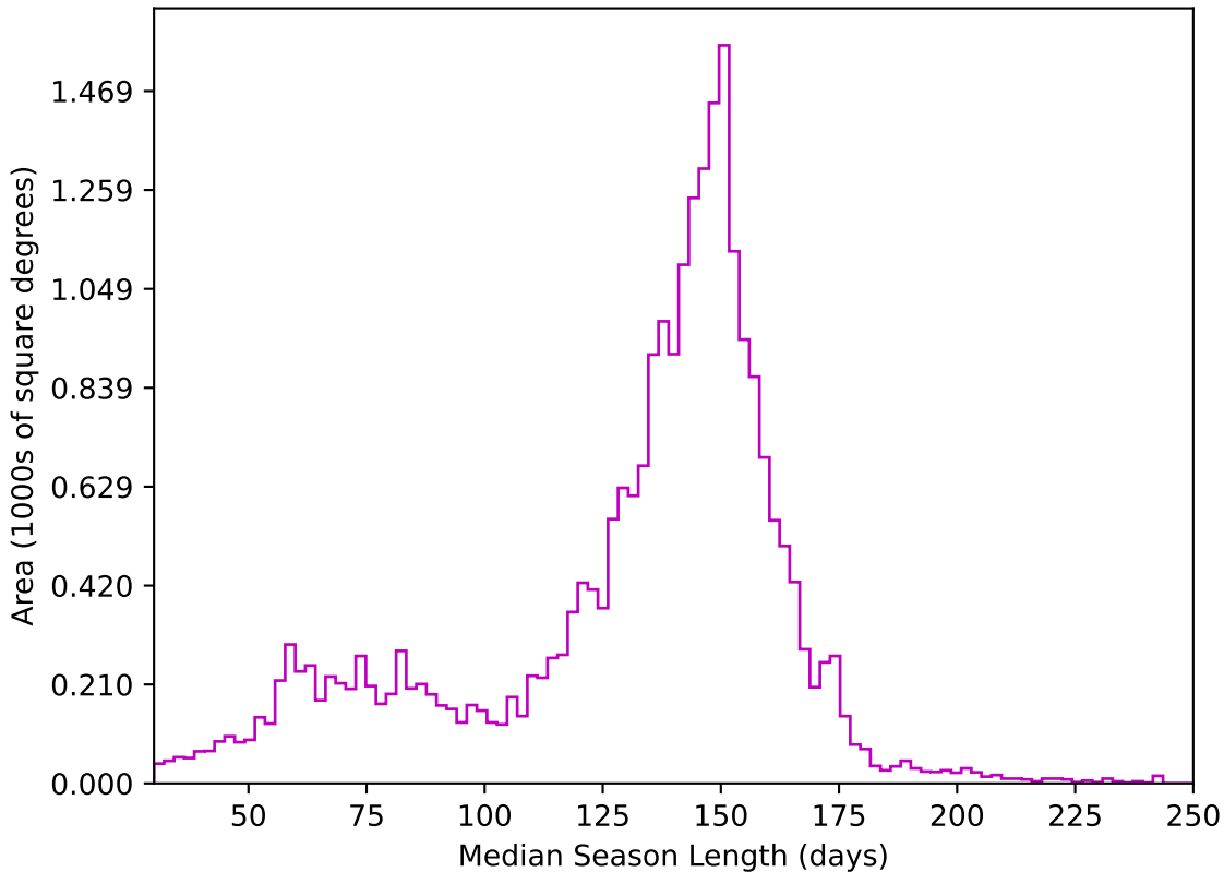
ddf_acor_sf15_lsf40_lsr50_v3.4_10yrs All sky z band: Median Season Length
