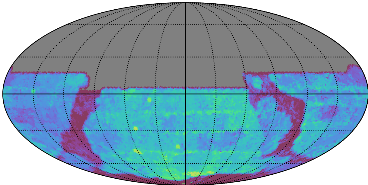
ddf_acor_sf15_lsf40_lsr50_v3.4_10yrs All sky y band: Median Season Length
