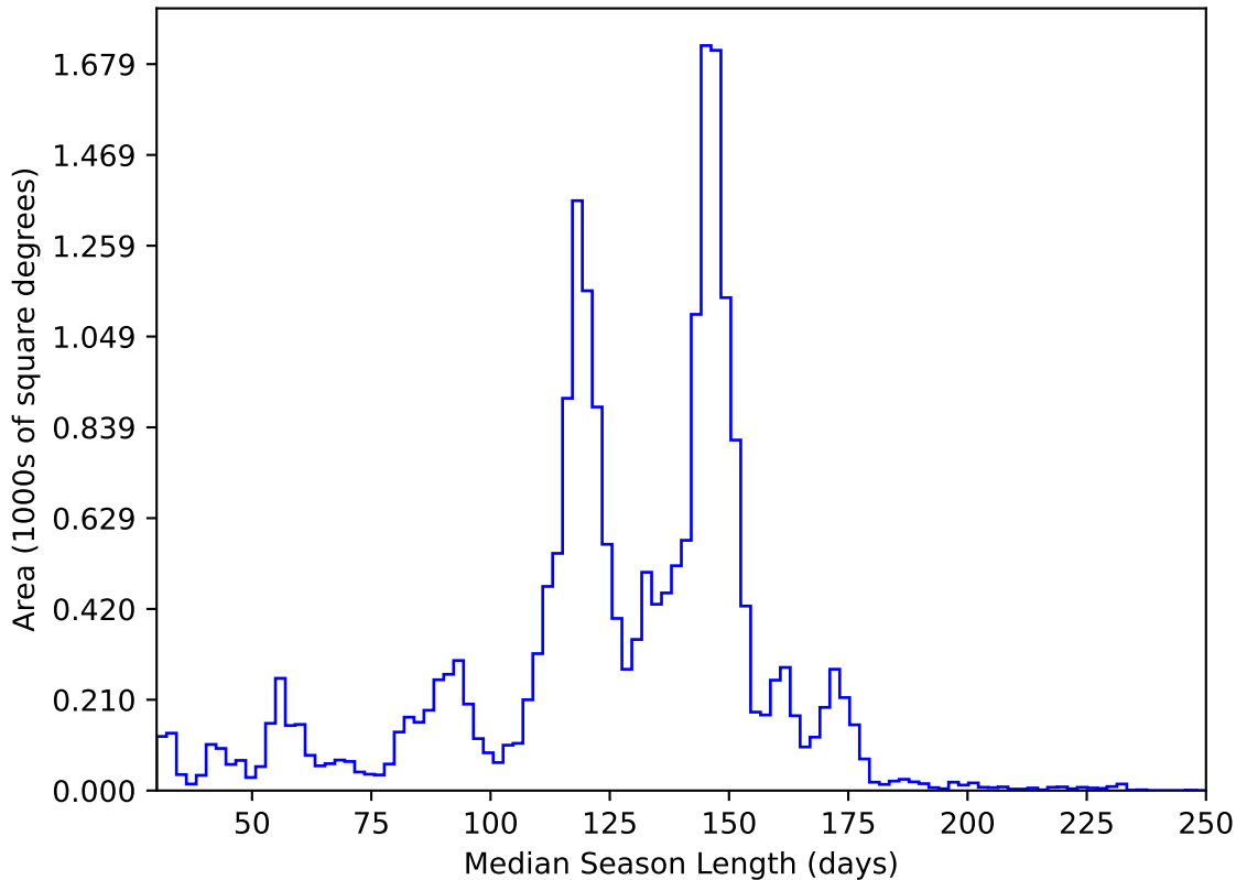
ddf_acor_sf15_lsf40_lsr50_v3.4_10yrs All sky y band: Median Season Length
