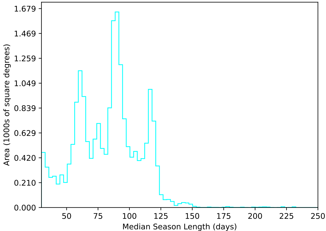
ddf_acor_sf15_lsf40_lsr50_v3.4_10yrs All sky u band: Median Season Length
