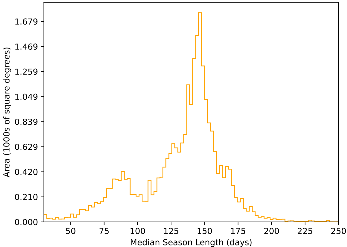
ddf_acor_sf15_lsf40_lsr50_v3.4_10yrs All sky r band: Median Season Length
