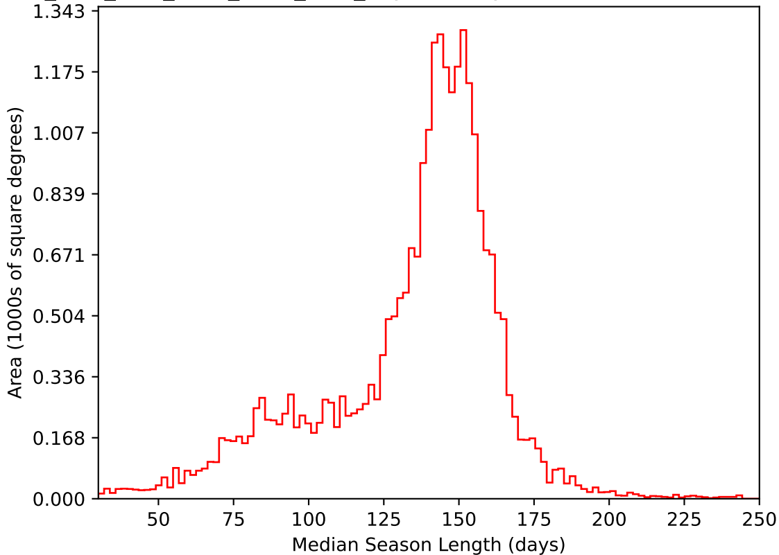
ddf_acor_sf15_lsf40_lsr50_v3.4_10yrs All sky i band: Median Season Length
