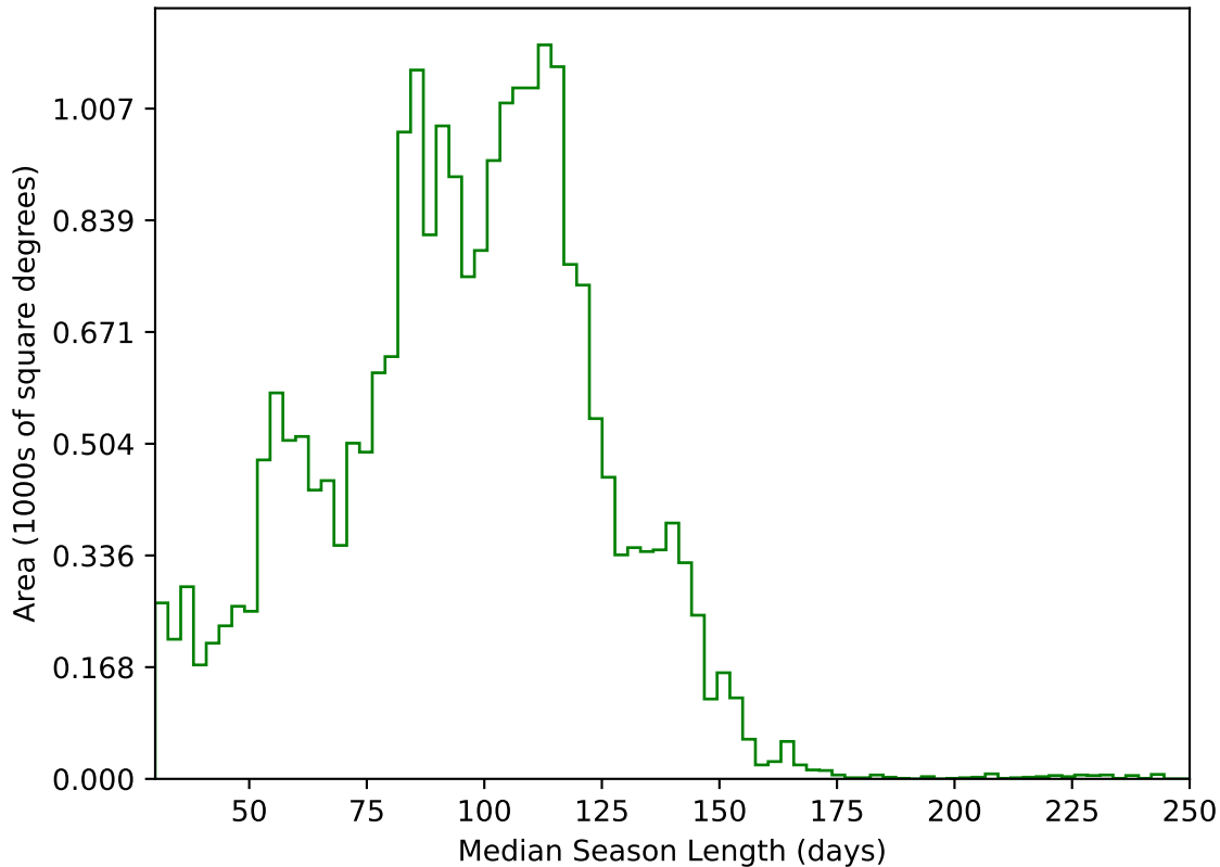
ddf_acor_sf15_lsf40_lsr50_v3.4_10yrs All sky g band: Median Season Length
