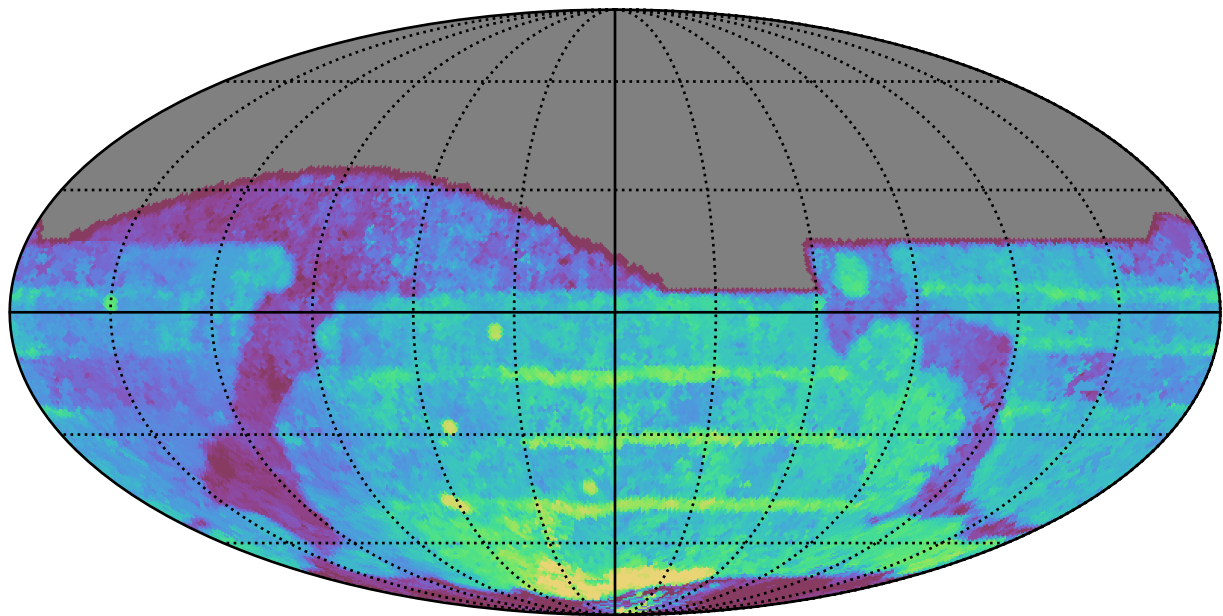
ddf_acor_sf15_lsf40_lsr50_v3.4_10yrs All sky all bands: Median Season Length
