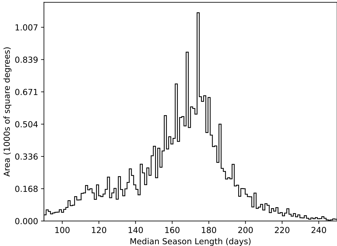
ddf_acor_sf15_lsf40_lsr50_v3.4_10yrs All sky all bands: Median Season Length
