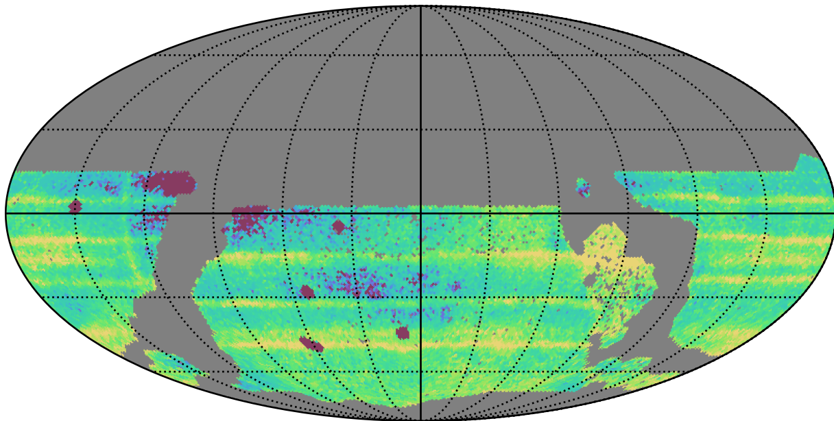
ddf_acor_sf15_lsf40_lsr50_v3.4_10yrs WFD: Median Intra-Night Gap
